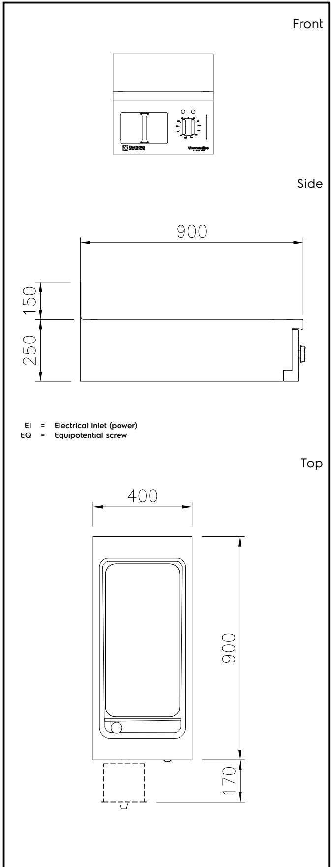
Cooking Range Line thermaline 90 Half Module Electric Fry Top, 1 Side - Marine USPHS only M2M
